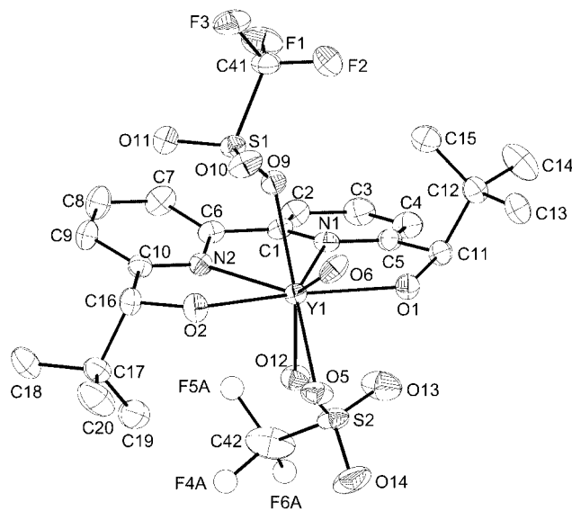
Figure 2. Crystal structure of the \text{Y}(\text{OTf})_3 -bipyridine 2 complex.
